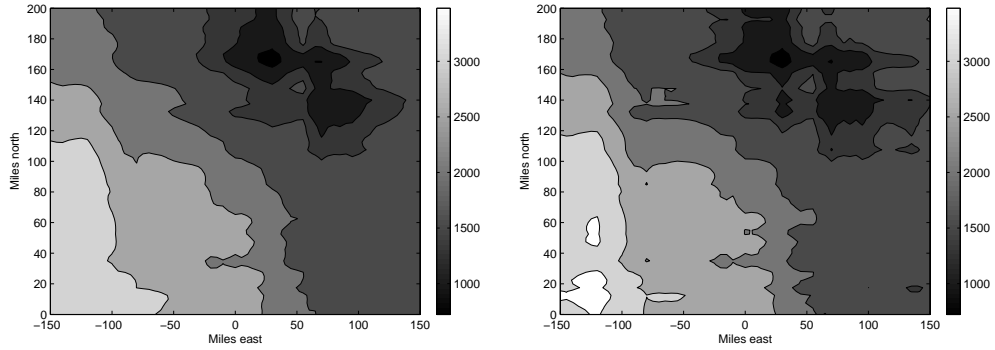
Figure 2: Kriging reconstruction of the Wolfcamp Aquifer data: predicted values with Bayesian (left) and WLS (right) black-box variogram estimates.
